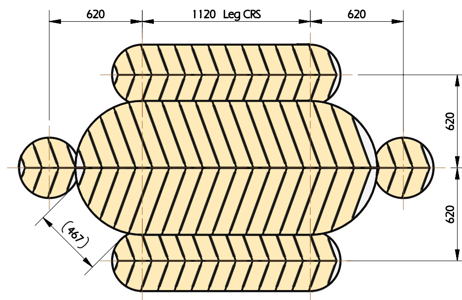
OTS-SM-001-2000-2B2S Orbella Table Setting - 2 Benches & 2 Stools
