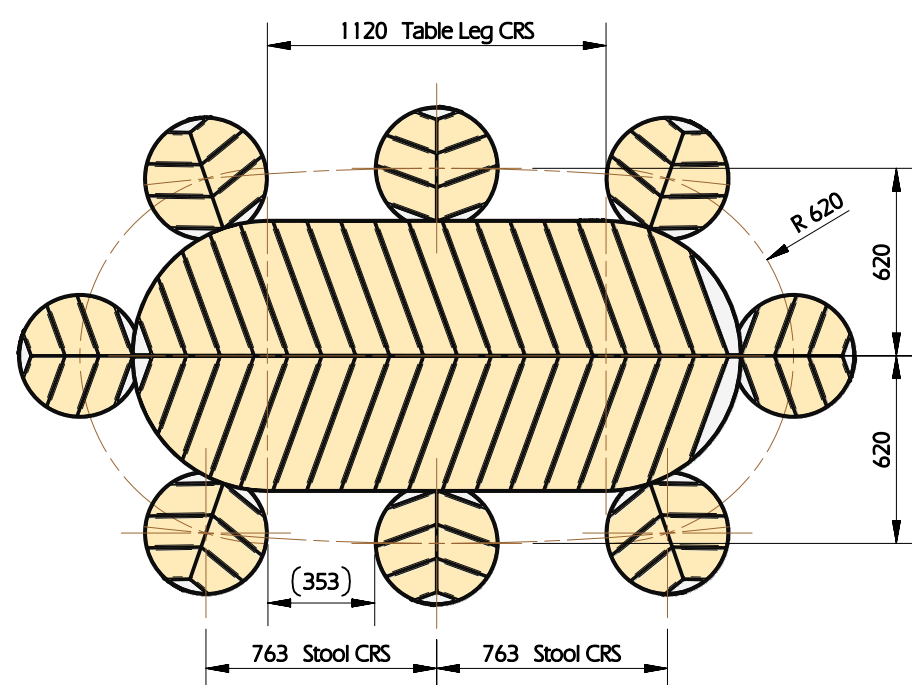
OTS-SM-001-2000-8S Orbella Table Setting - 8 Stools
