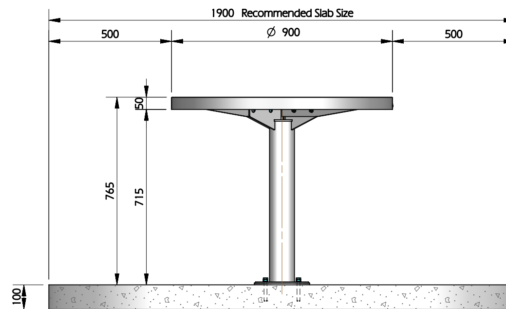
SIDE VIEW SCALE: NTS
