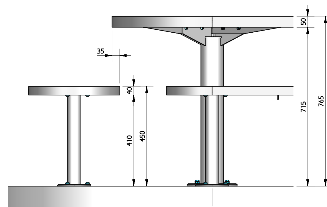
TYPICAL TABLE SETTING PROFILE
