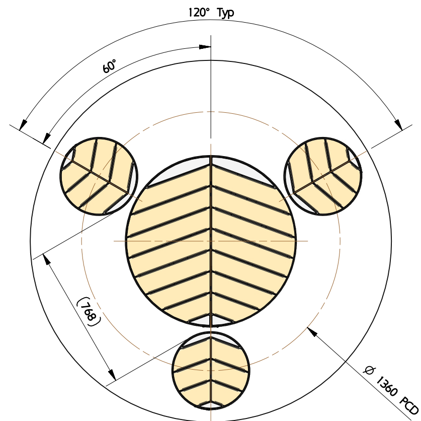
ORTS-SM-001-D900-3S Orbella Ø 900 Round Table Setting - 3 Stools
