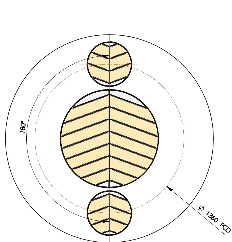
ORTS-SM-001-D900-2S Orbella Ø 900 Round Table Setting - 2 Stools
