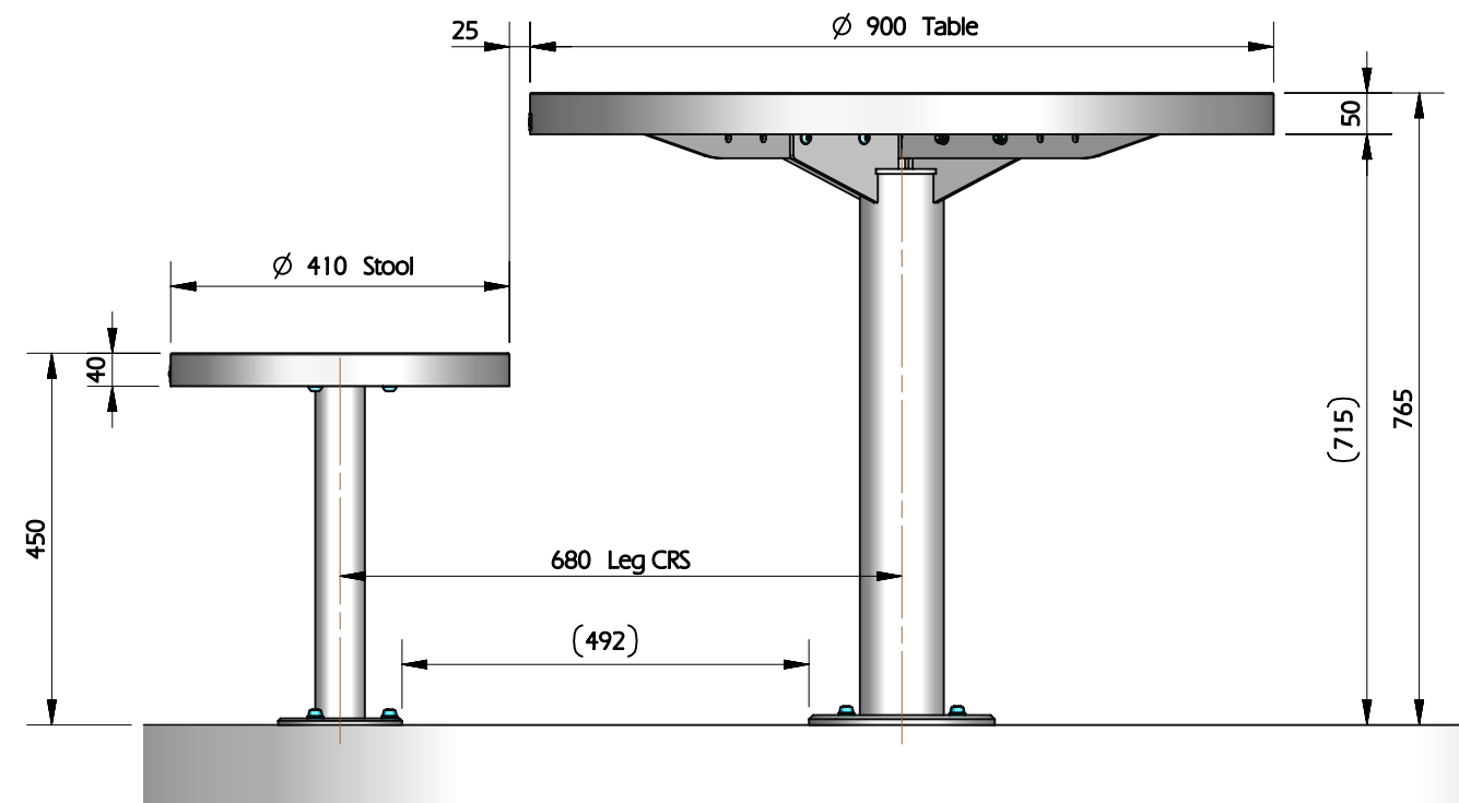
TYPICAL SIDE VIEW
