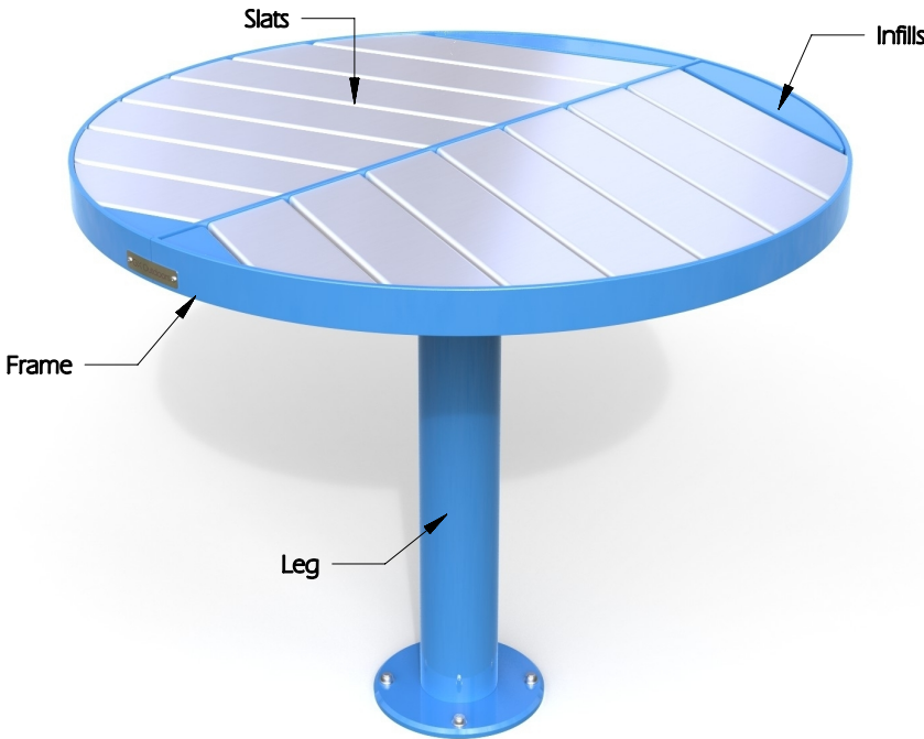
FINISH OPTION: Deluxe (DEL) Slats: Anodized Aluminium Frame, Legs & Infills: Powder coated Aluminium
