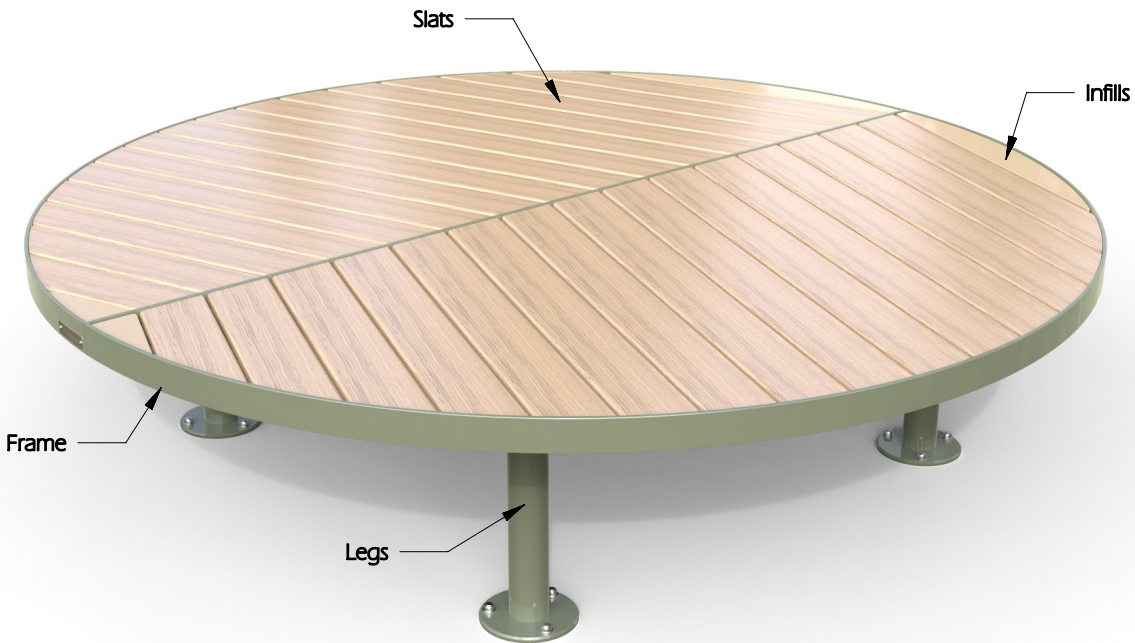
FINISH OPTION: Timber Image (TIM) Slats: Timber Image Aluminium Frame, Legs & Infills: Powder coated Aluminium
