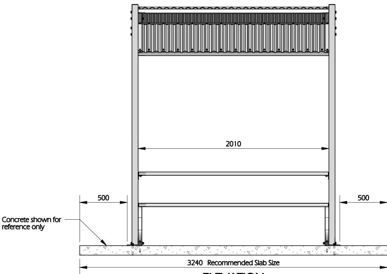
ELEVATION SCALE 1:25
