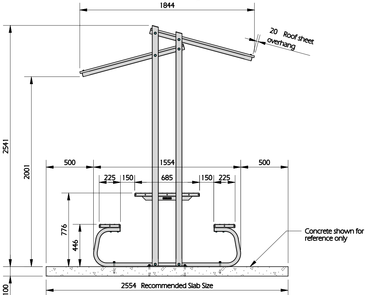
SIDE VIEW SCALE 1:25
