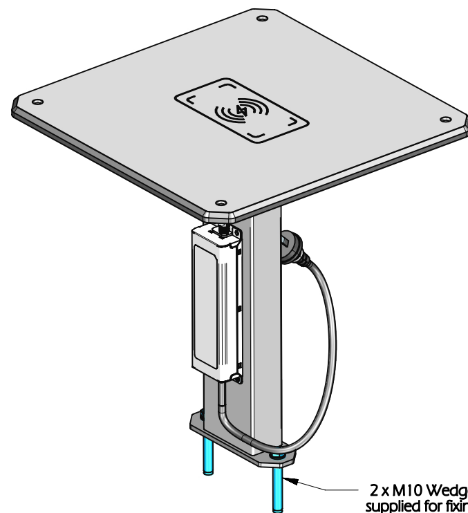
PICTORIAL VIEW - AS SUPPLIED
