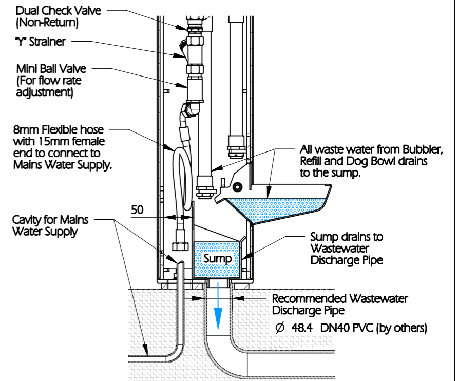
CONNECTION & WASTEWATER DISCHARGE DETAILS SECTION A-A
