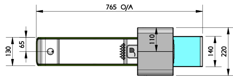
TOP VIEW SCALE 1:10
