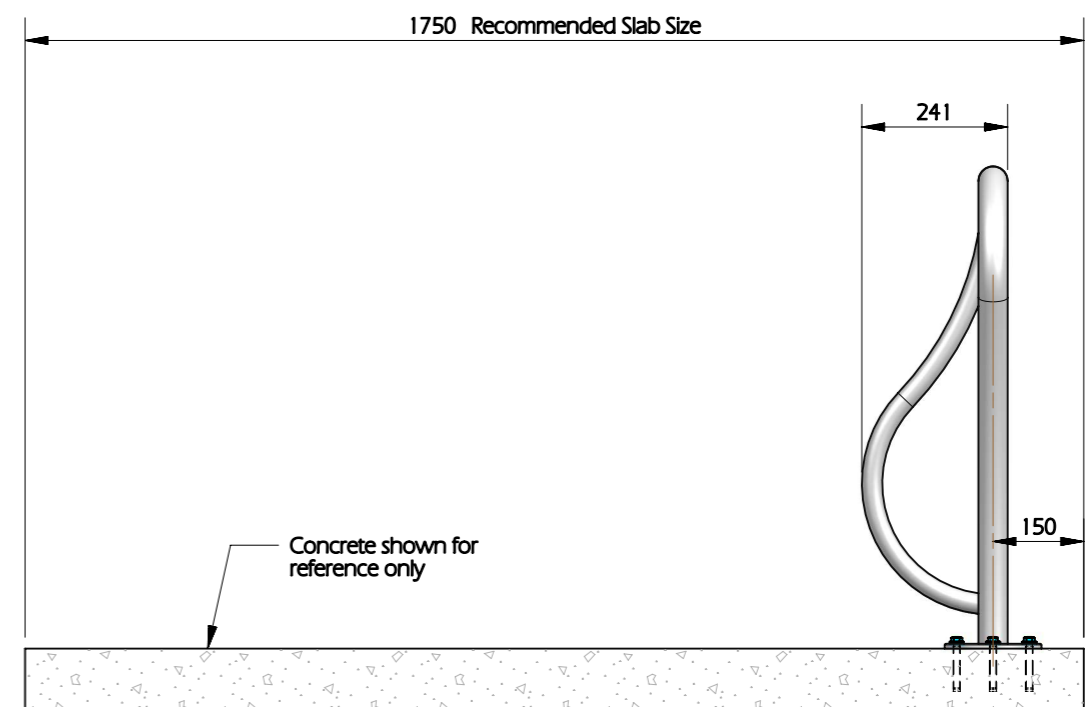
SIDE VIEW
