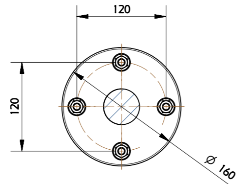
FOOTPRINT SECTION A-A SCALE 1:5
