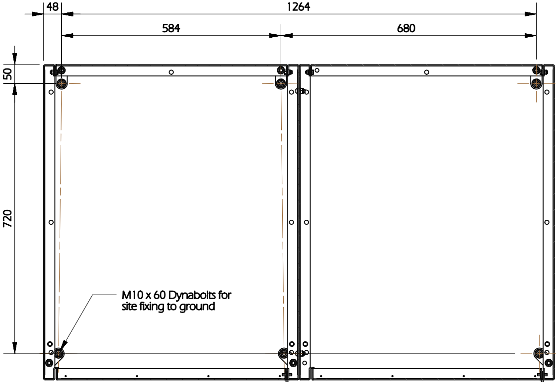
FOOTPRINT SECTION A-A SCALE 1:10
