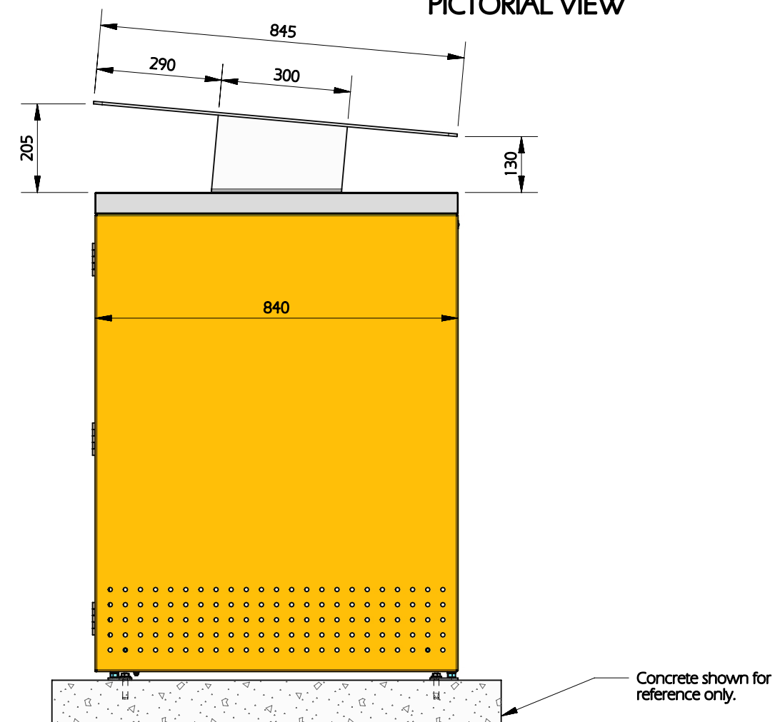
SIDE VIEW SCALE: NTS
