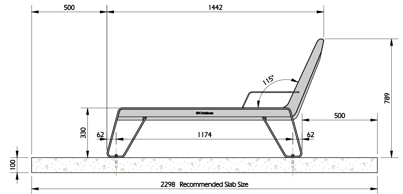
SIDE VIEW SCALE 1:15
