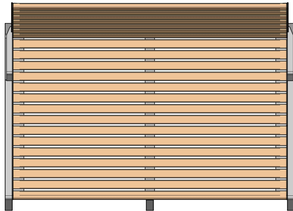
TOP VIEW SCALE 1:15
