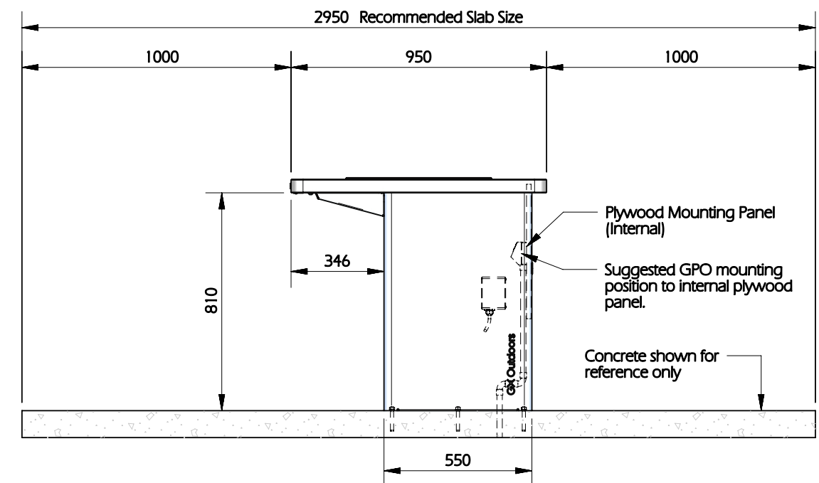
SIDE VIEW SCALE 1:20
