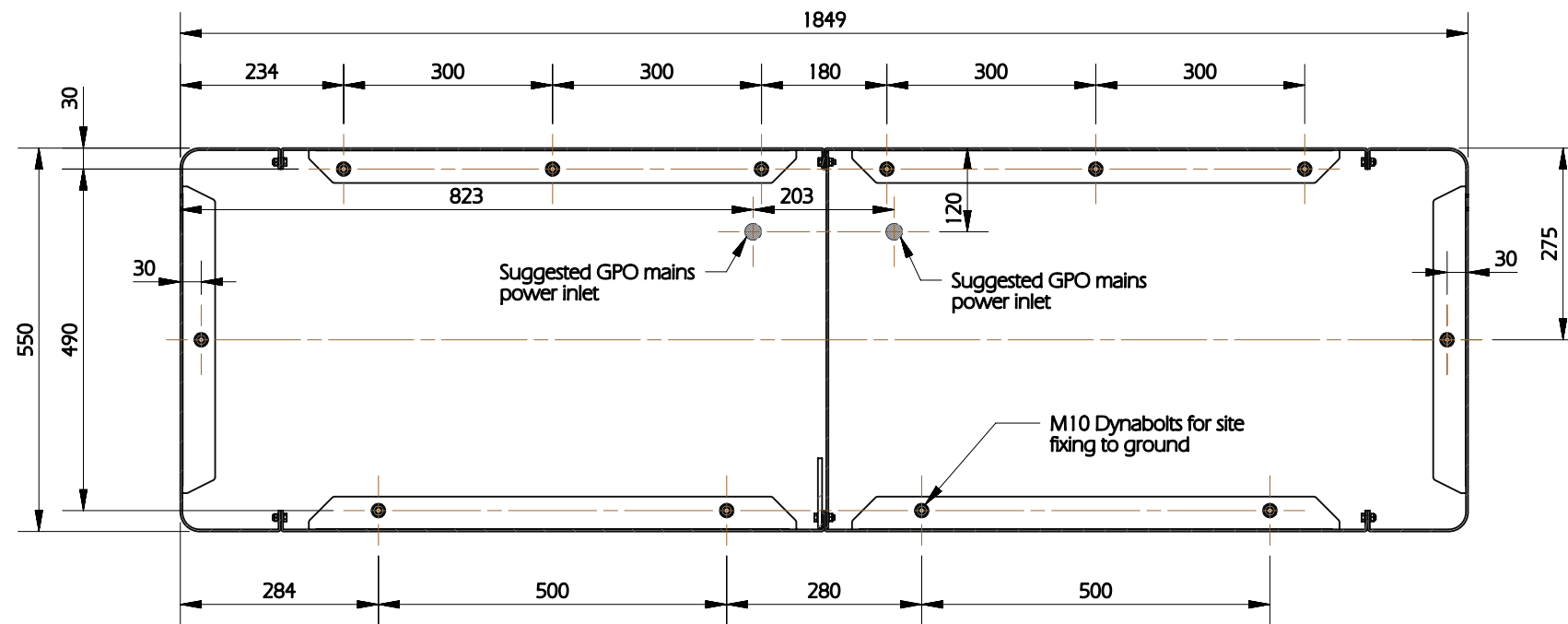
FOOTPRINT SECTION A-A SCALE 1:10
