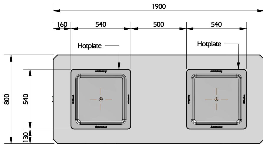
TOP VIEW SCALE 1:20
