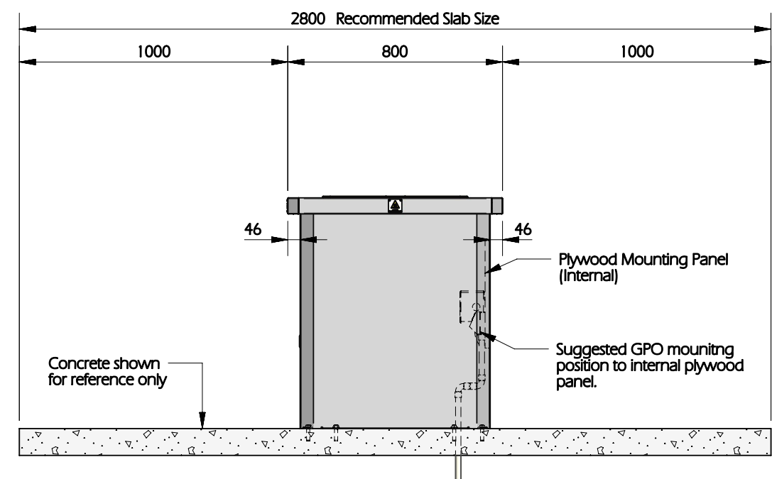
SIDE VIEW SCALE 1:20
