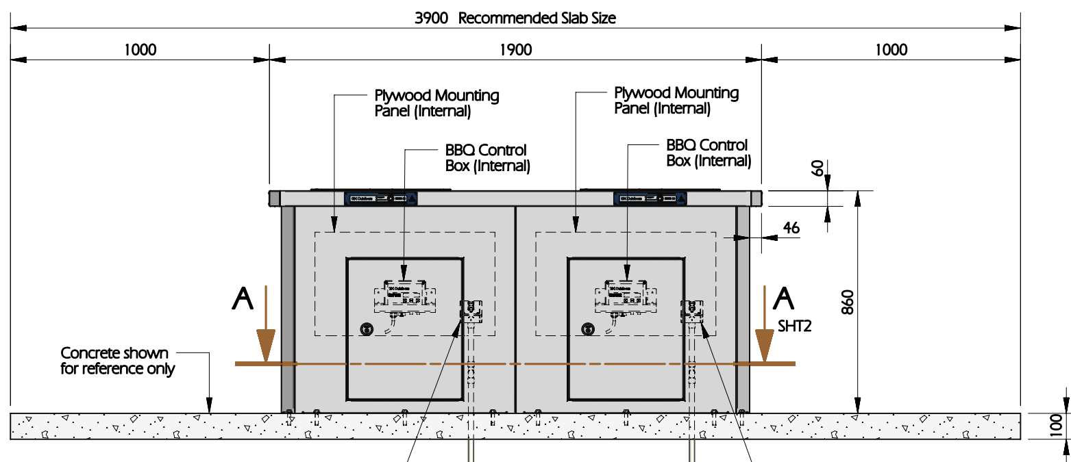
ELEVATION (FOOTPRINT ON SHT2) SCALE 1:20
